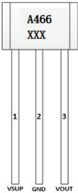
TO92S
