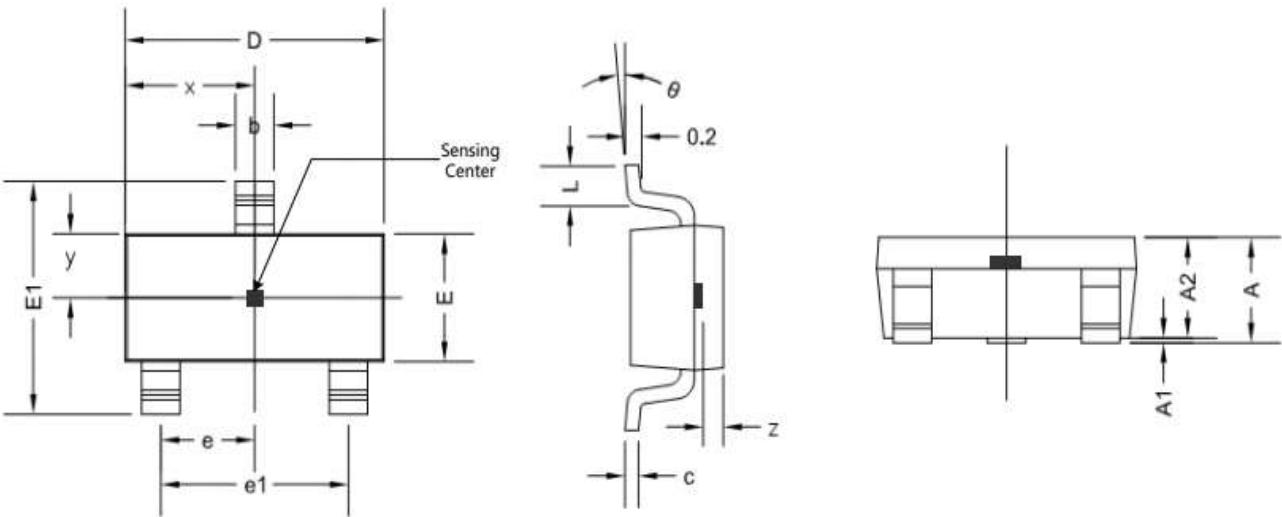
SOT23 (Thin Outline) 尺寸
